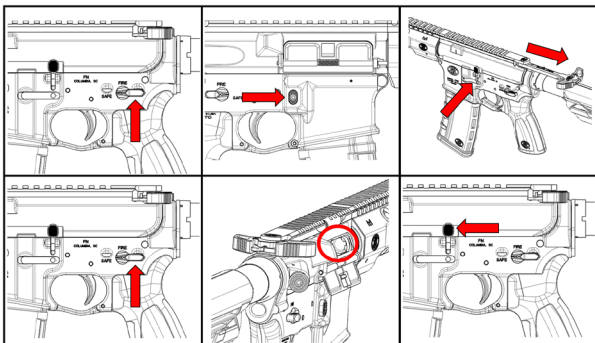
Unloading the FN15.
