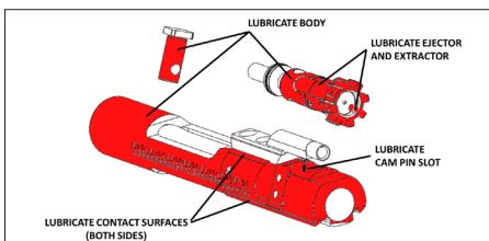
Lubrication of the bolt carrier assembly.
