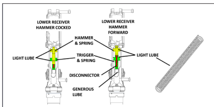
Lubrication of the lower receiver.
