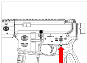
Selector - FIRE position.
