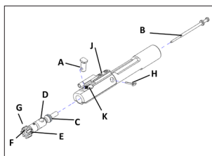
Bolt carrier assembly inspection.
