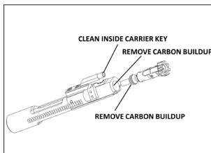
Bolt carrier cleaning.
