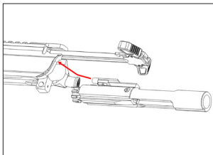
Install bolt carrier assembly.
