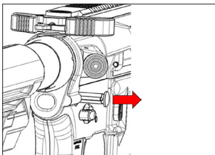
Pull takedown pin.
