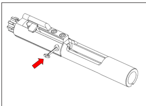
Install firing pin retaining pin.
