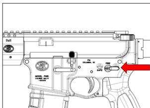
Selector - SAFE position.
