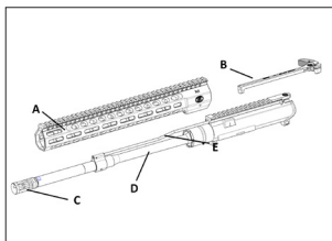
Upper receiver inspection.
