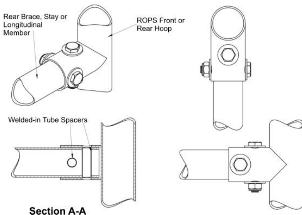
Figure LK17 Tube Joins
