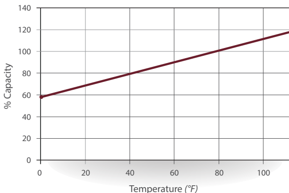
Temperature versus Capacity
