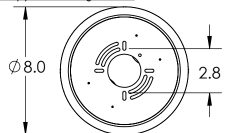
Canopy Mounting Detail
