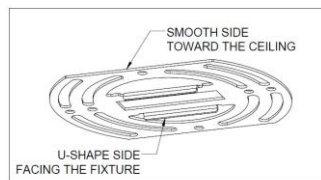
PROPER ORIENTATION OF GEM BAR FOR INSTALLATION
