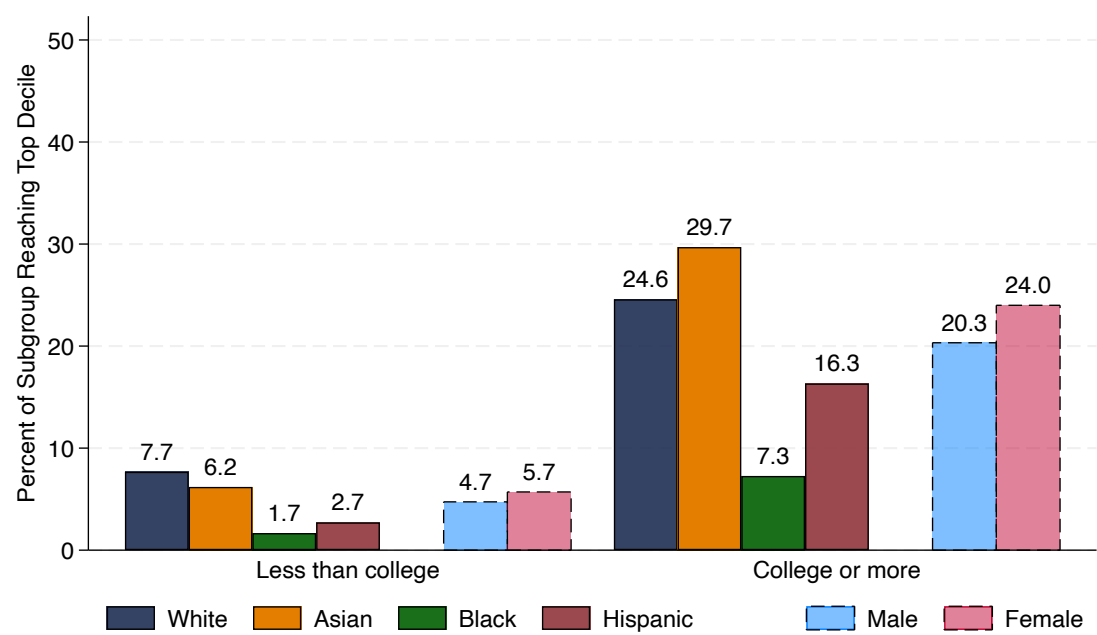
(a) Math
