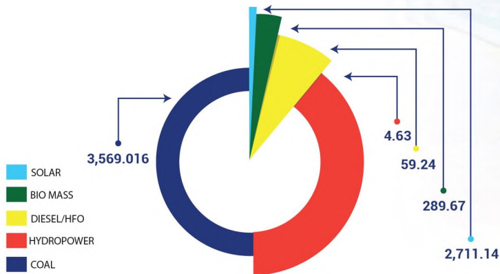
Energy Sent Out In GWh By Type Of Generation
