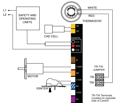
Figure 7 – 7565 (for replacement of R7184B) Valve-on delay only (no motor-off delay)
