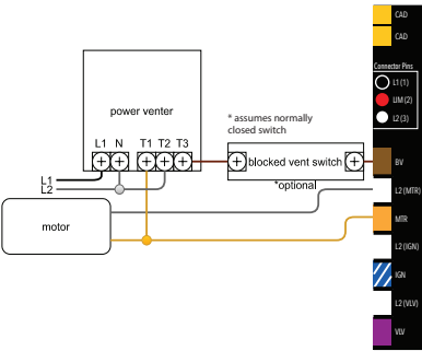
Figure 14 - 120Vac Combustion Air Proving Wiring
