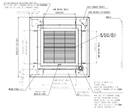
PLA-AENL ① ② A B C D E F 12~18 REFRIGERANT PIPE #2.5 (FLARE) CONNECTION 1/4" REFRIGERANT PIPE #2.7 (FLARE) CONNECTION 1/2" 241 79-1/20 250 C1-5/32 76 C2-63/64 76.5 C3-1/64 265/101-7/16 250/103-25/32 DR MORE DR LESS 24~40 REFRIGERANT PIPE #5.0 (FLARE) CONNECTION 3/8" REFRIGERANT PIPE #5.88 (FLARE) CONNECTION 5/8" 281 C1-1/16 291 C1-2/32 79.5 C1-1/8 79.5 C1-1/8 305/121 450/127-5/32 DR MORE DR LESS
