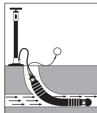
Step 4. Removal
