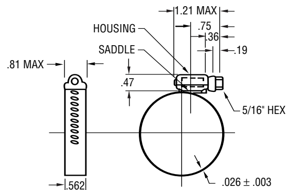
CLAMP DETAIL
