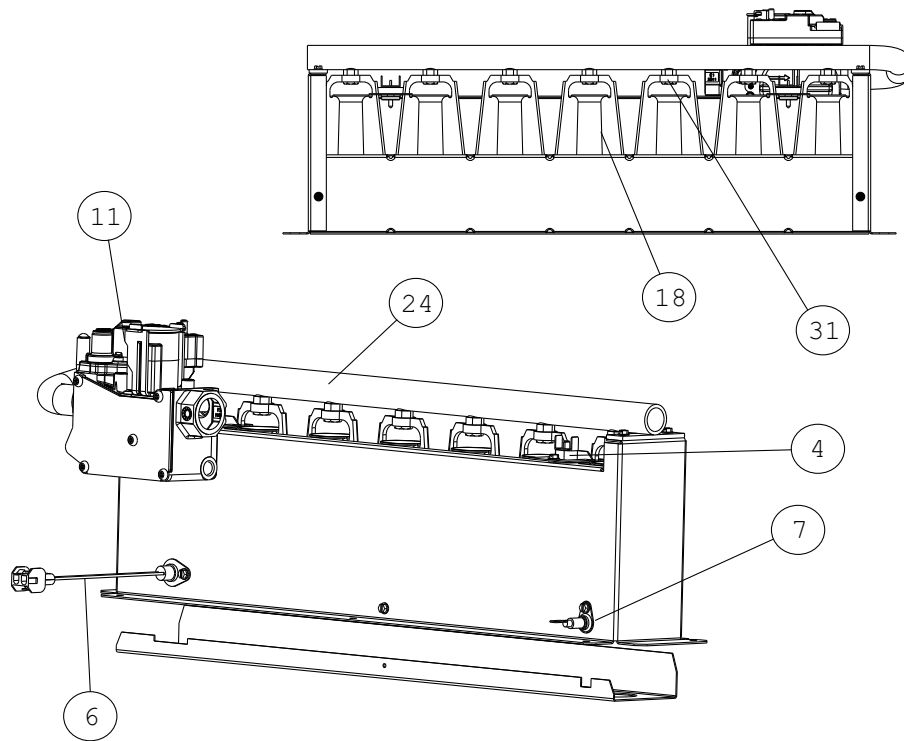
Figure 3: GAS CONTROLS
