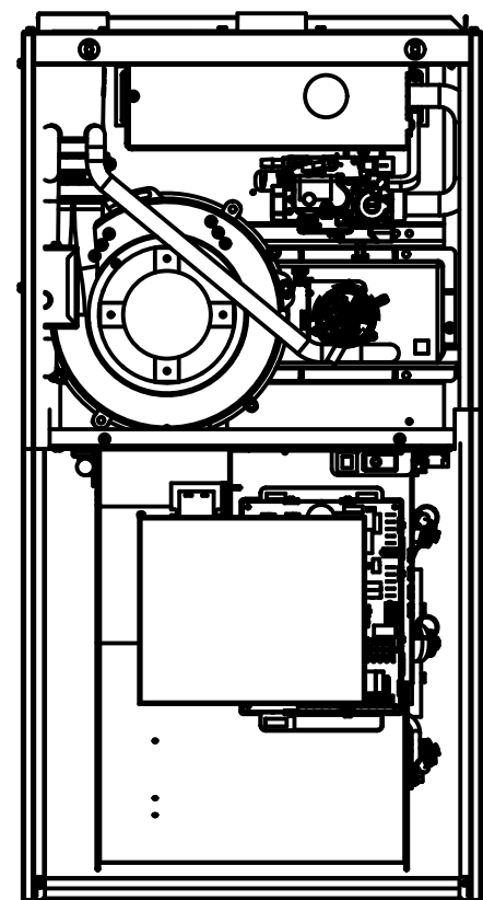
WIRE ROUTING
