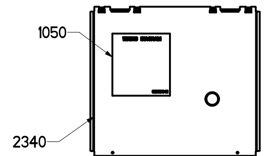
INNER DOOR ACCESS PANEL REAR VIEW
