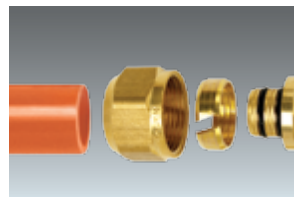
SST20 Compression
