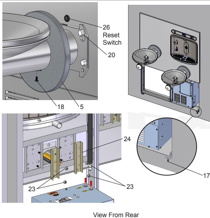
Figure 4 - Fountain Installation
