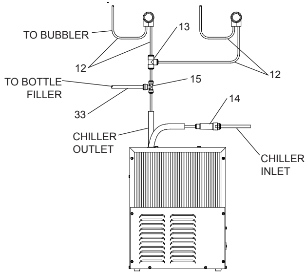
Figure 2 - EZWS-ERPB Tube Routing
