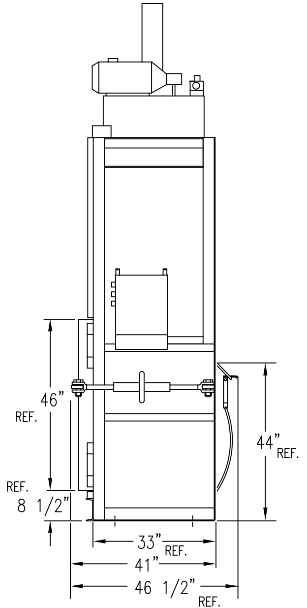
RIGHT SIDE
