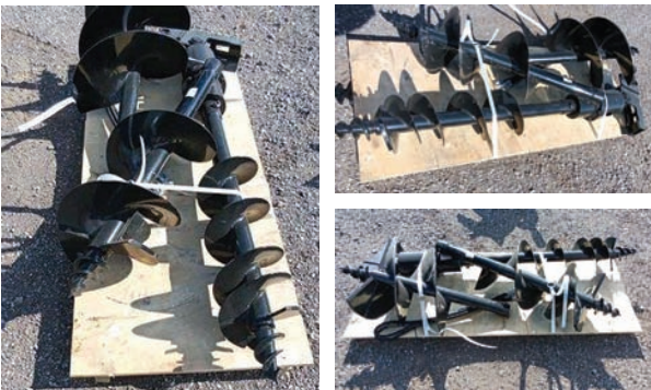
New 2024 GIYI Qty 3 Skid Steer Loader Attachments 8" auger, with 12" /16" auger rod, fits a 1-3 ton excavator, pin diameter 1"
