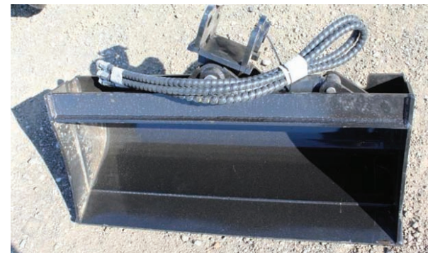
New 2024 MIVA 32" Titling Bucket fits a 1-3 ton excavator, pin diameter 1"
