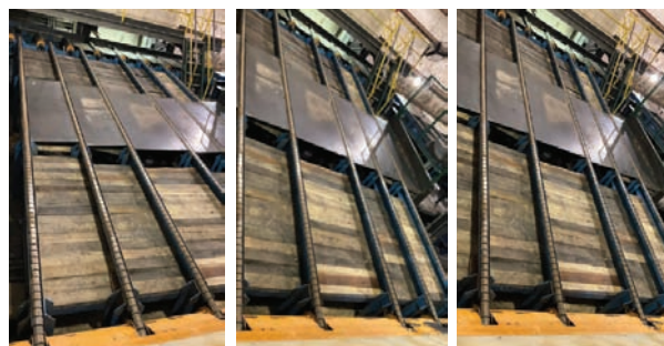
Transfer Deck (Part of an entirety) # of Strands: 6. Chain Type: H78B rooftop. Drive Type: Electric. Overall Dimensions: 14' x 27'. Features and Notes: Slant deck section for side loading, no sprockets on one end.
