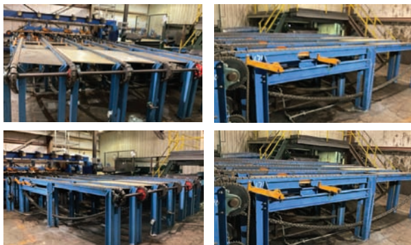
Transfer Deck (Part of an entirety) # of Strands: 6. Chain Type: H78B rooftop. Drive Type: Electric. Overall Dimensions: 17' x 15'. Features and Notes: No shaft or sprockets on one end, board stops.
