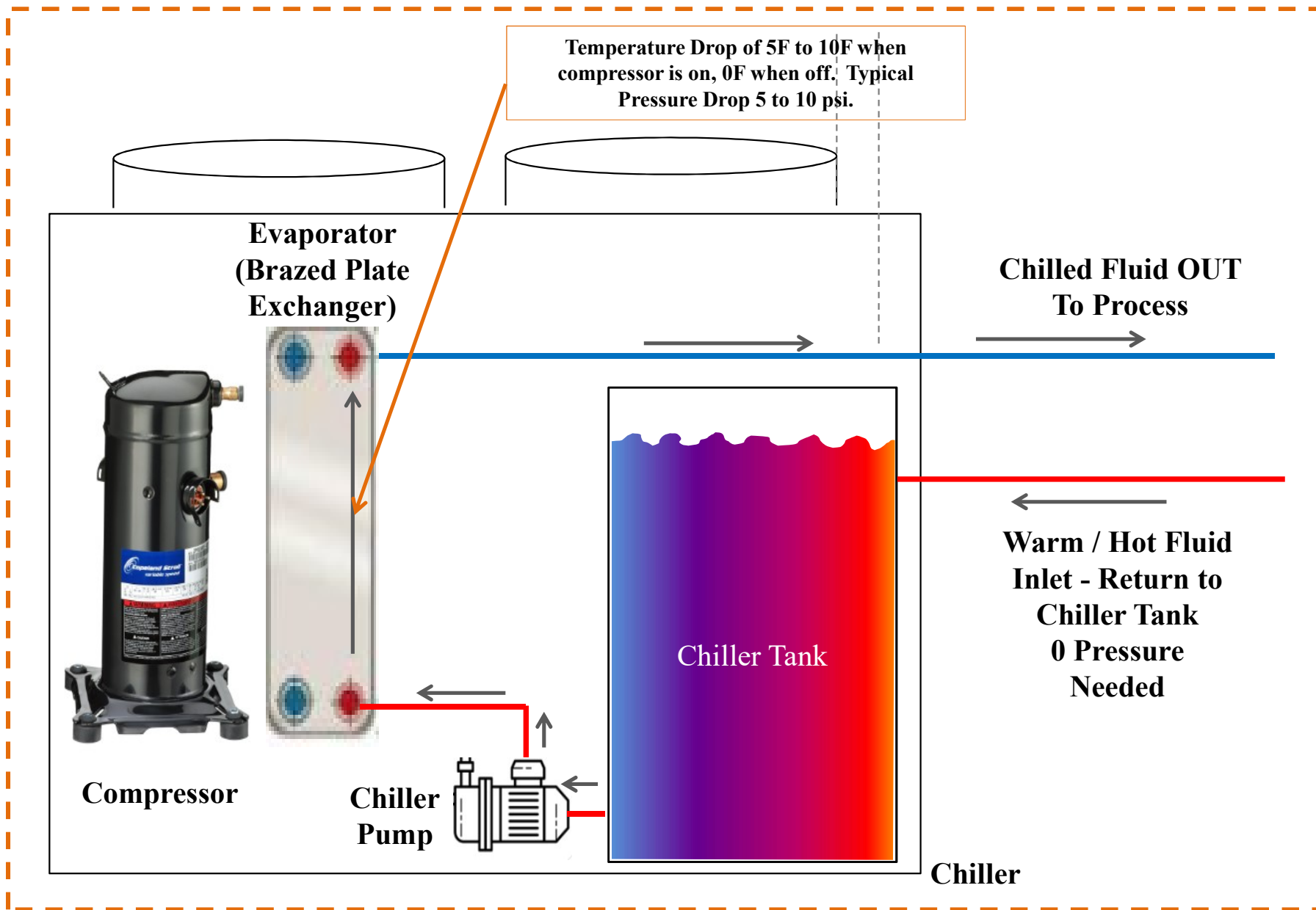
Standard Closed Loop Chiller w/ Plate Type Evaporator. Configured for warm water return and 0 psi return Flow.
