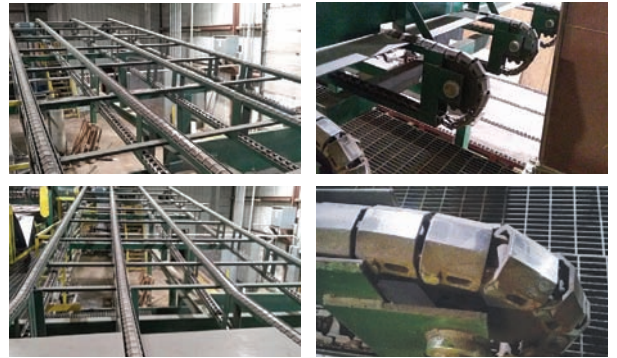
4 Strand Green Chain — Specifications & Features — Make: na. Drive Type: Electric. # of Strands: 4. Overall Dimensions: 9'x36'. Chain Type: H78B Rooftop chain. — Seller Statement — No support legs.
