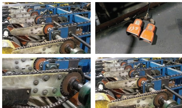
4 Strand Transfer Deck with Tipple Arms — Specifications & Features — Make: na. Drive Type: Electric. # of Strands: 4. Overall Dimensions: 8'x10'.
