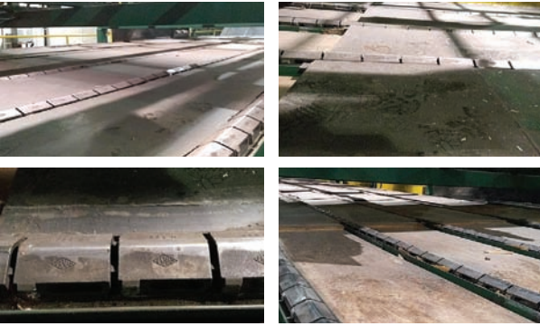
5 Strand Green Chain — Specifications & Features — Make: na. Drive Type: Electric. # of Strands: 5. Overall Dimensions: 11'x44'. Chain Type: H130 Rooftop.
