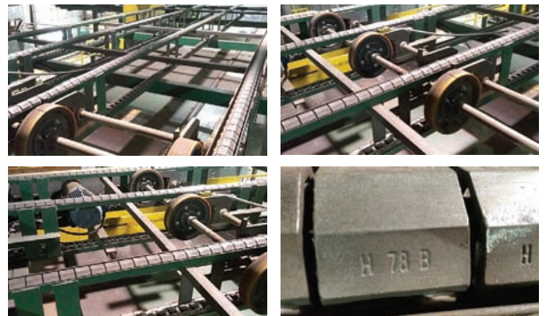
4 Strand Green Chain — Specifications & Features — Make: na. Drive Type: Electric. # of Strands: 4. Overall Dimensions: 9'x30'. Chain Type: H78B Rooftop. — Seller Statement — No support legs.
