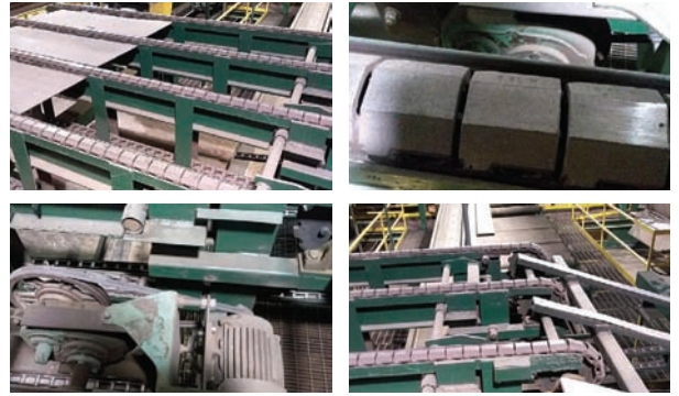
5 Strand Transfer Deck — Specifications & Features — Make: na. Drive Type: Electric. # of Strands: 5. Overall Dimensions: 8'x11'. Chain Type: H78B Rooftop.
