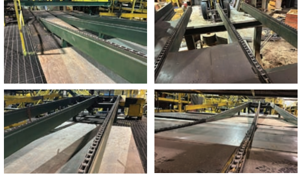
Inclined Transfer Deck
