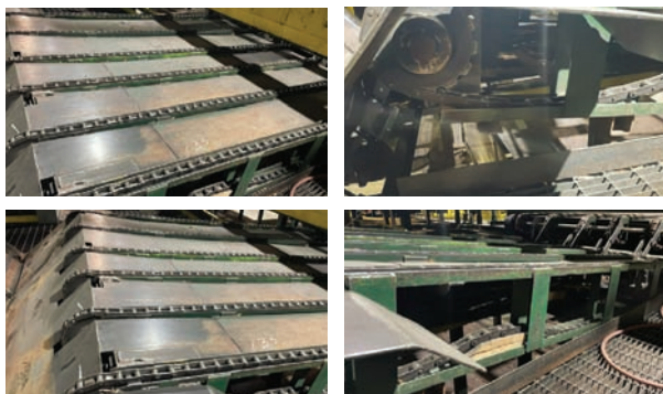
6 Strand Transfer Deck — Specifications & Features — Make: na. Drive Type: Electric. # of Strands: 6. Overall Dimensions: 106"x128". — Seller Statement — Good condition
