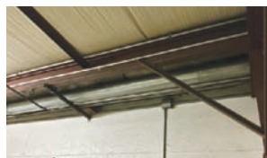
Blower, Pipe and Cyclone — Description — 18" blower and cyclone, 7" steel pipe, some 4" branches, approximately 100' total
