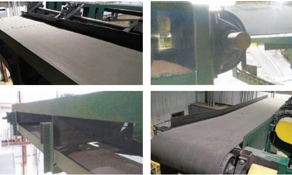
Belt Conveyor — Specifications & Features — Drive Type: Electric. Length: 15'. Overall Width: 26". Belt Width: 22 1/2".
