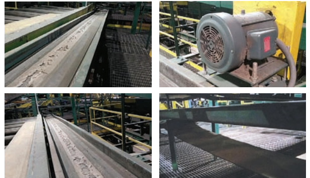
Belt Conveyor — Specifications & Features — Drive Type: Electric. Length: 60'. Overall Width: 2'. Belt Width: 17".
