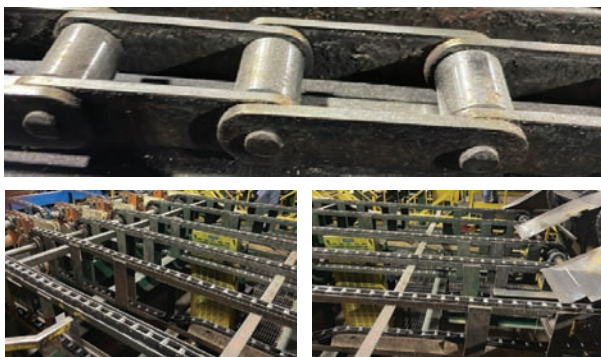
6 Strand Transfer Deck — Specifications & Features — Make: na. Drive Type: Electric. # of Strands: 6. Overall Dimensions: 106"x116".
