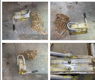
Magnet and Chain — Description — Permanent magnet 1000 kg capacity, 1/4" chain
