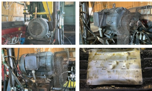
Electric Motor — Specifications & Features — Make: na. Horsepower: 150. Phase: 3 Phase. Frame Size: 443-0595. RPM: 1185.
