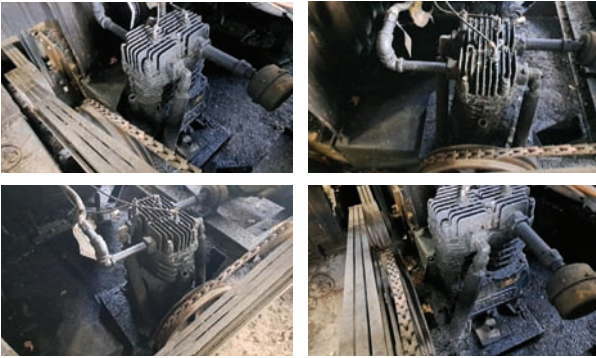
Quincy Air Compressor — Description — Single head
