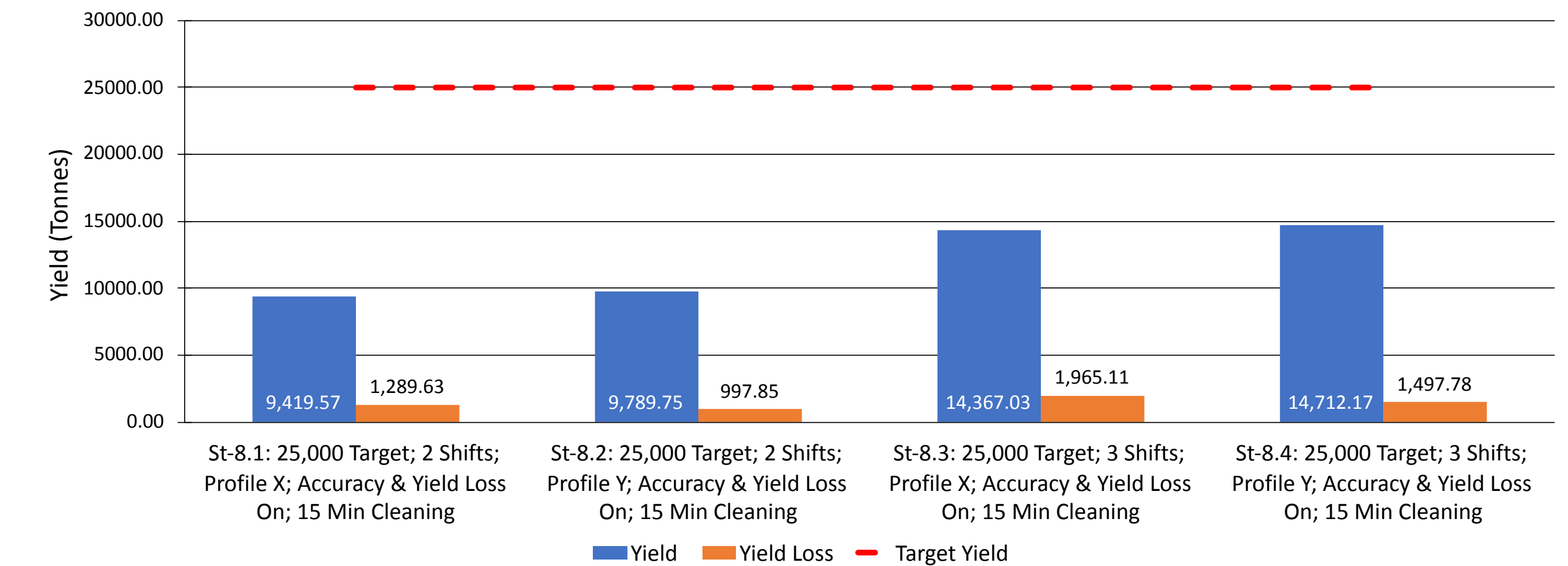
Figure 60: Maximum system yield profile for St8.1 - St8.4 (with constraints)
