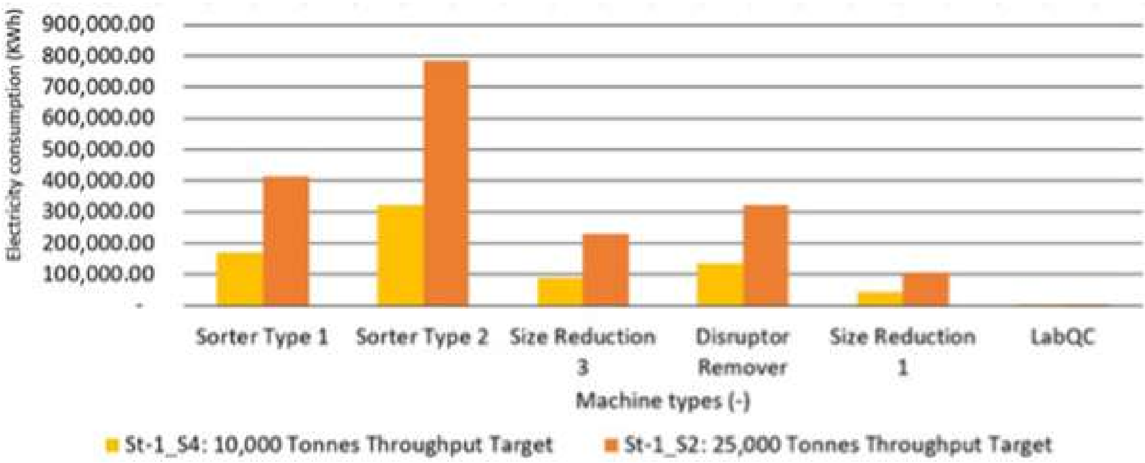
Figure 44: Effect of target throughput increase to machine electricity consumption
