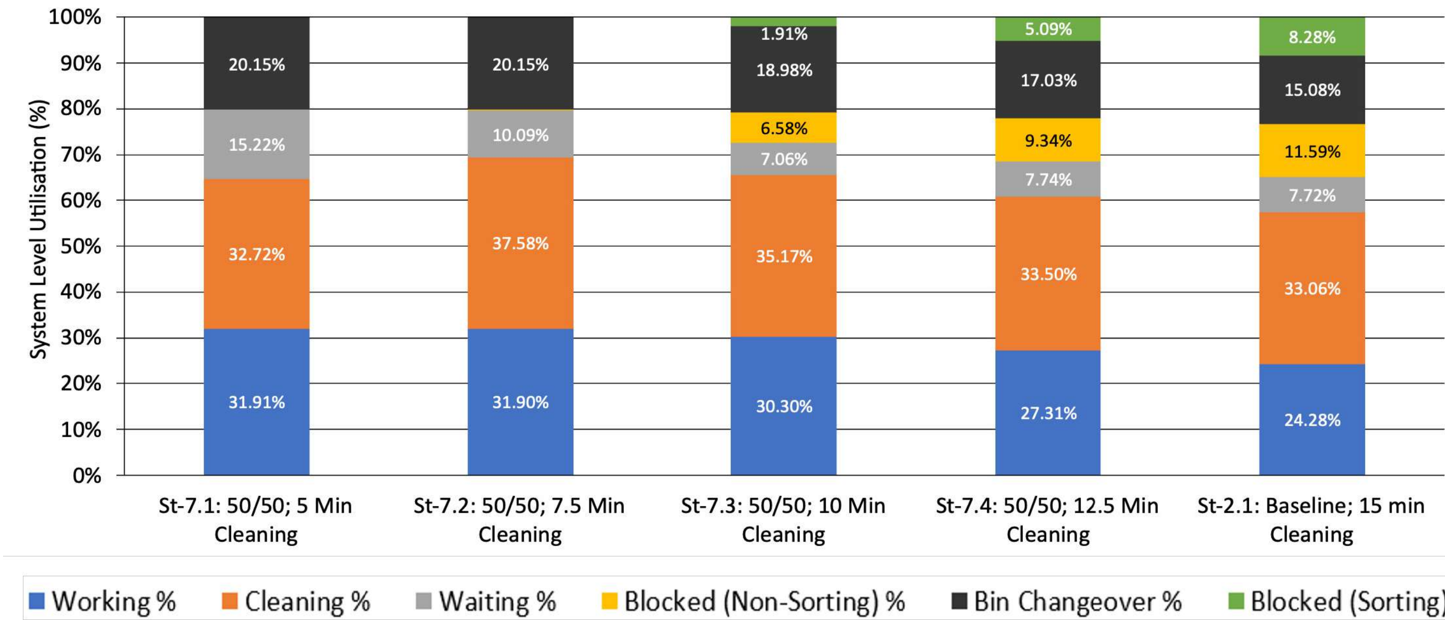
Figure 59: System level utilisation
