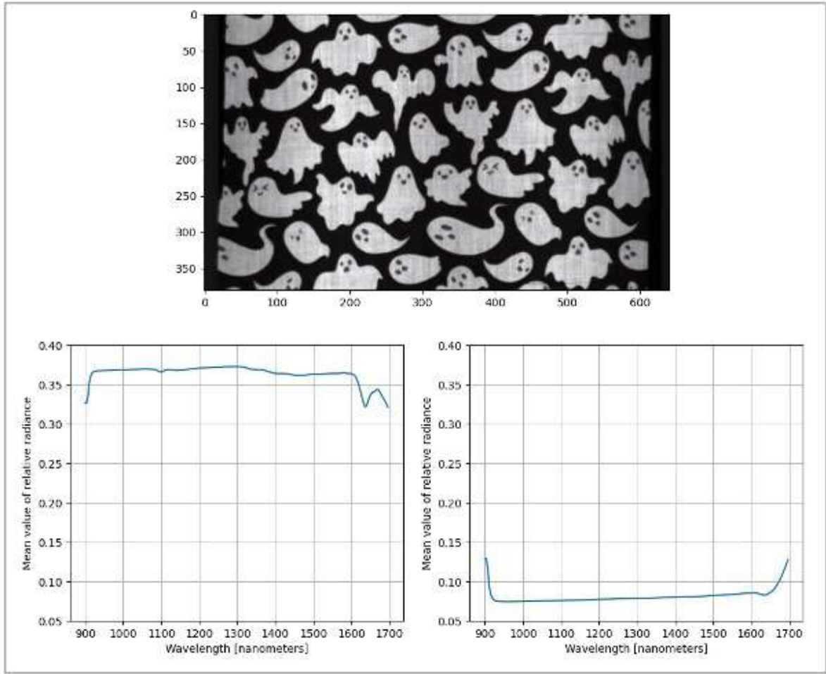
Image 19: Automatic collection of 100 spectral samples
