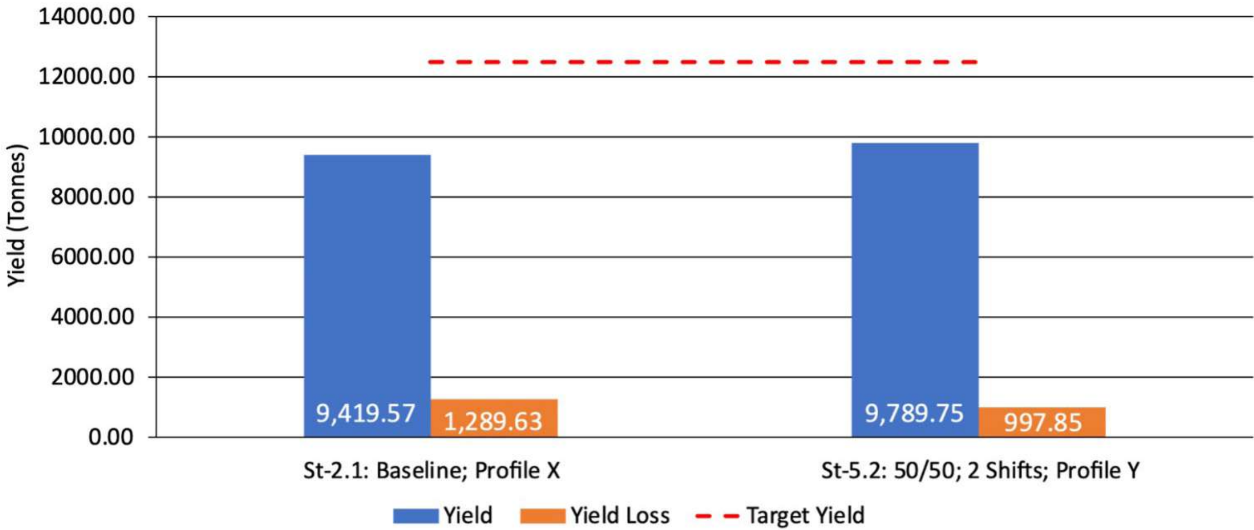
Figure 54: System yield profile for St-5.2 compared to baseline
