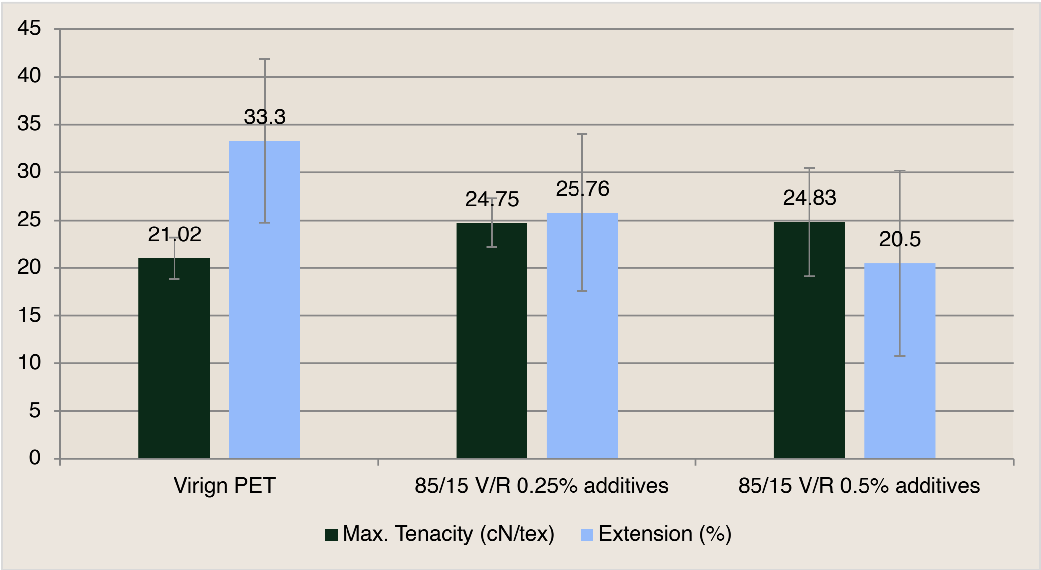
Figure 81: Tenacity and elongation at break for spun PET multifilaments
