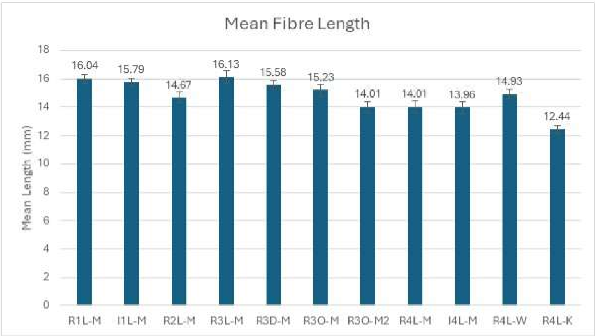
Figure 92: Cotton fibre analysis: Mean fibre lengths
