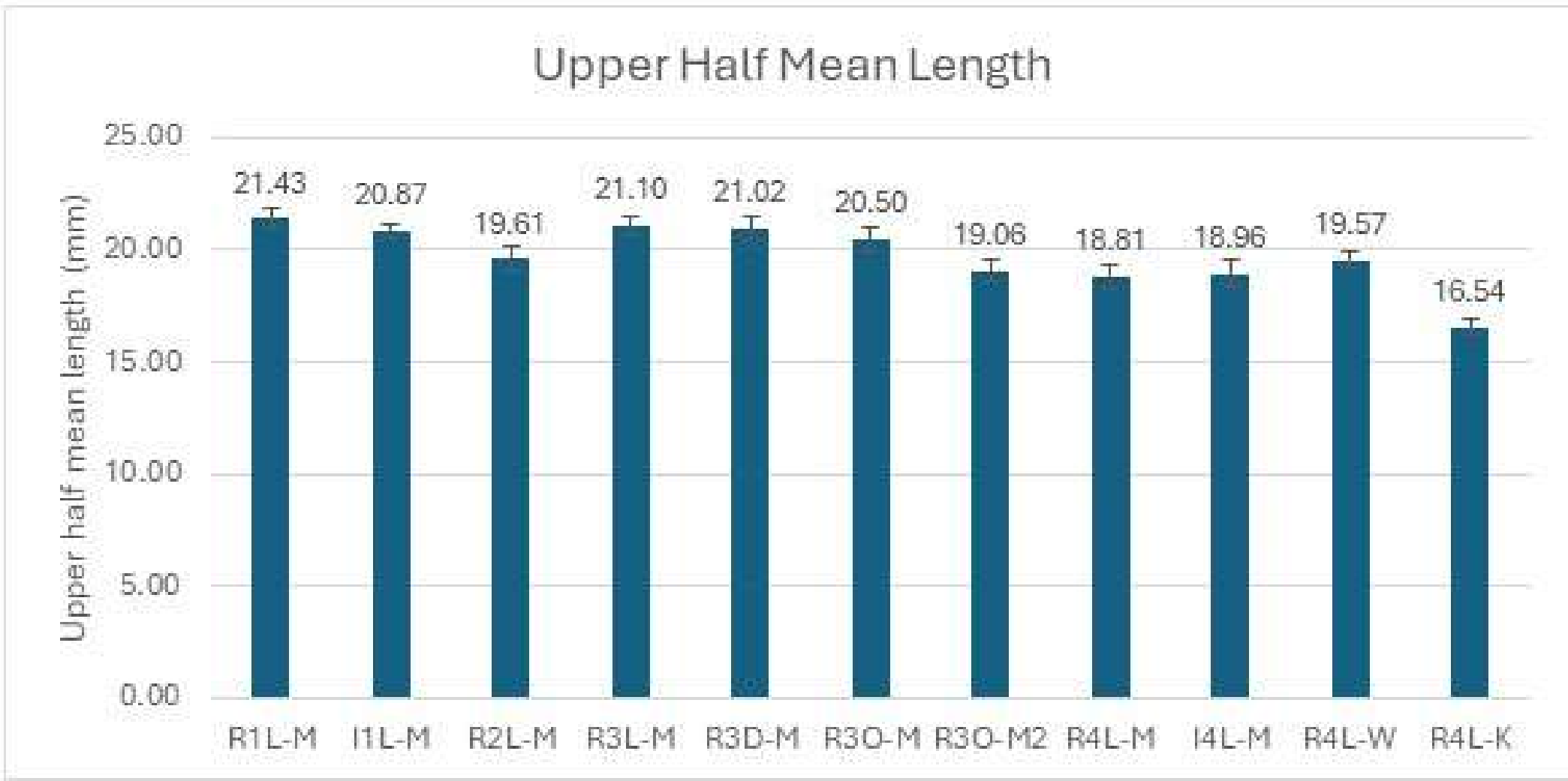
Figure 93: Cotton fibre analysis: Upper half mean length
