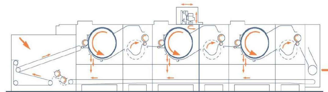
Figure 31: Tearing machine schematic
