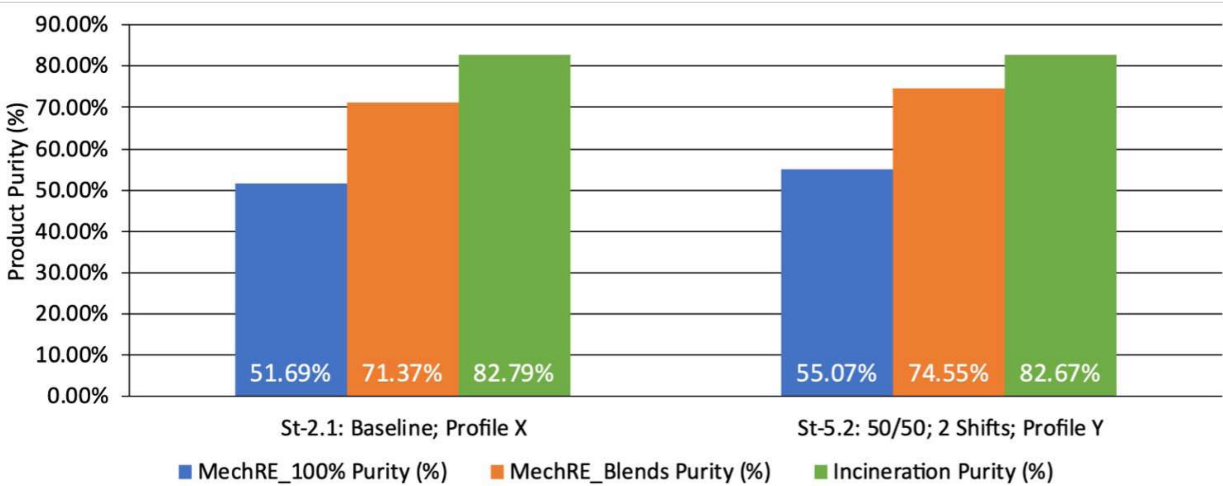
Figure 55: Product purity profile for S5.2 (2-shift, 50:50 blend) compared to baseline
