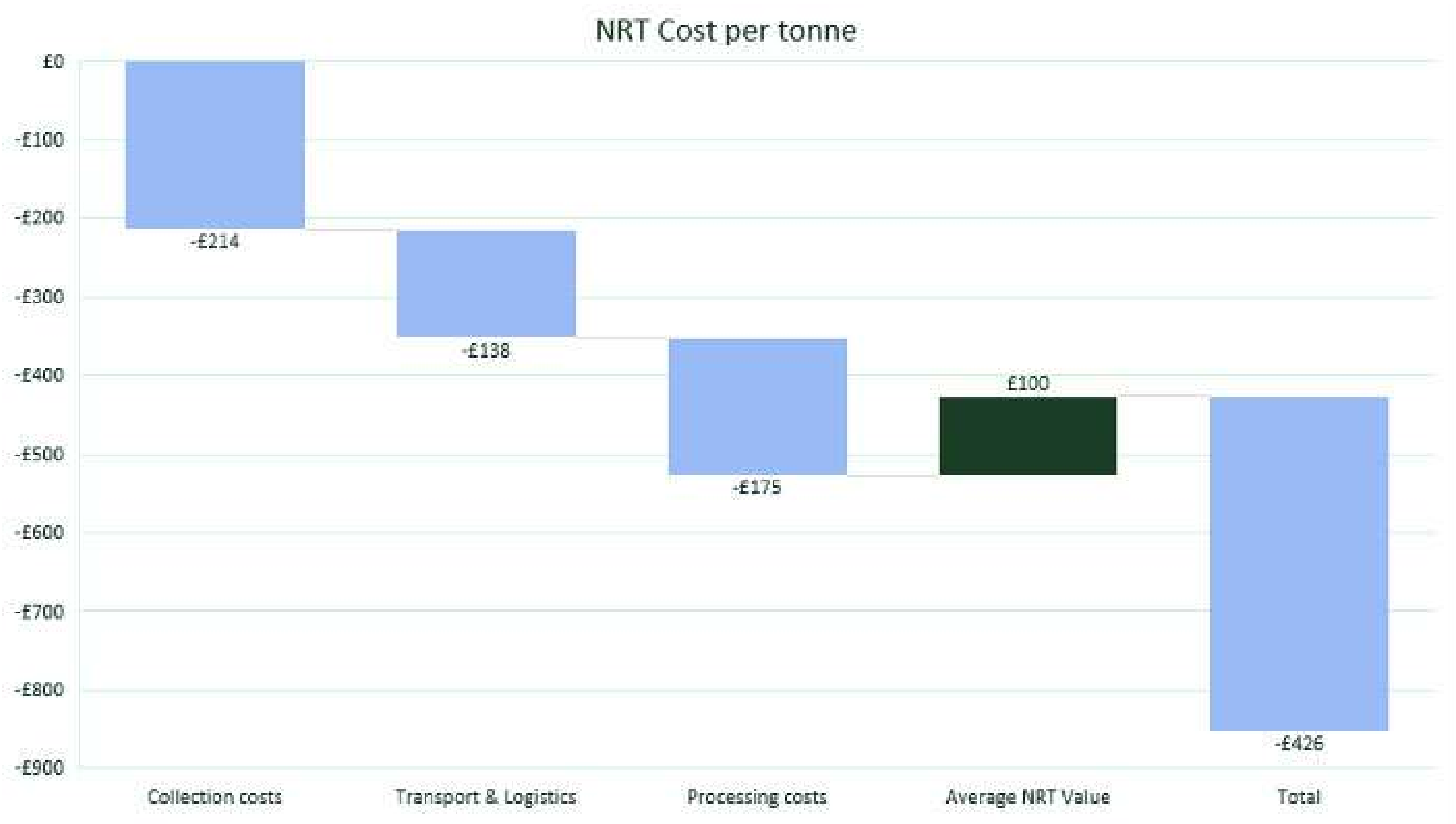
Figure 147: Current NRT cost overview under manual sorting
