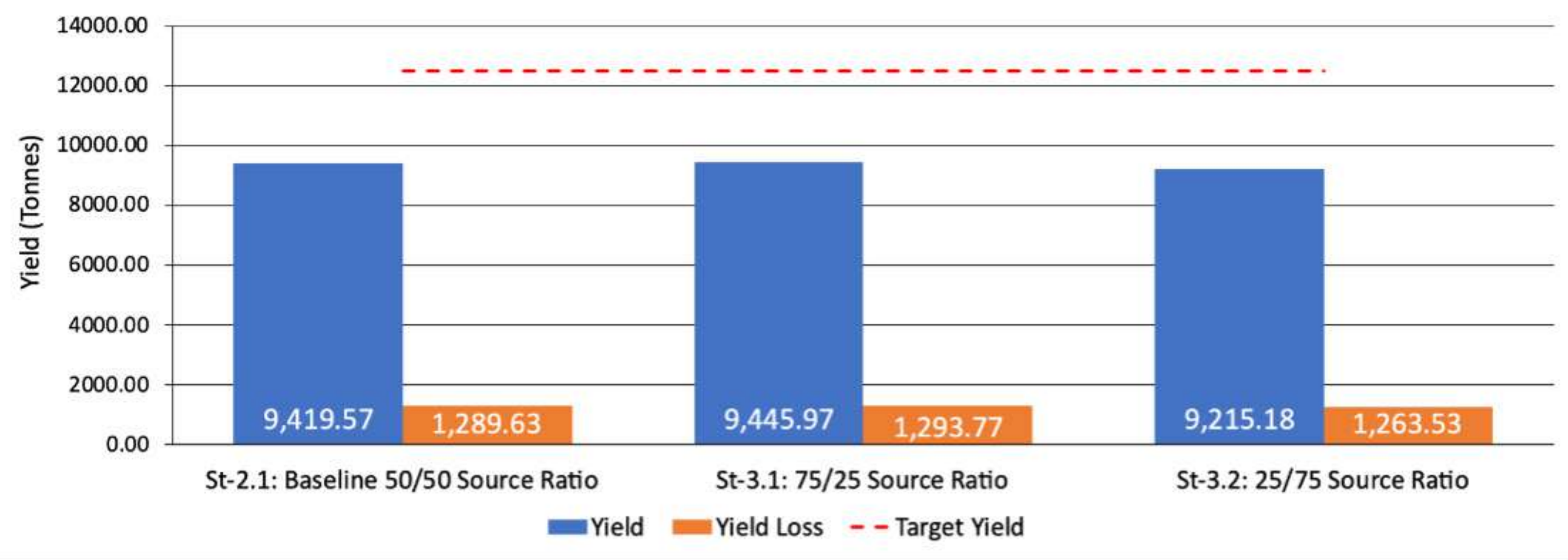
Figure 51: System yield profile for the baseline (S3.1 and S3.2)
