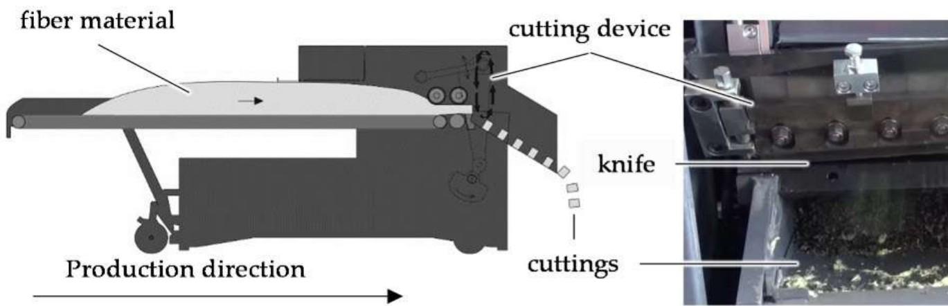
Image 13: Schematic of guillotine cutting
