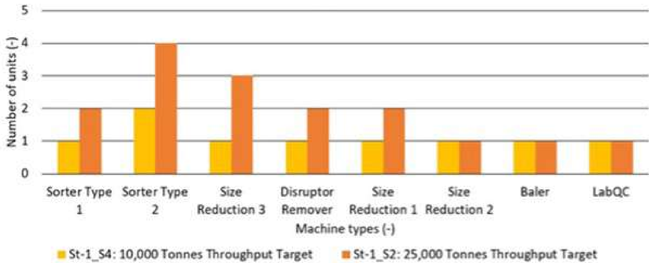
Figure 42: Effect of target throughput increase to number of units per machine type
