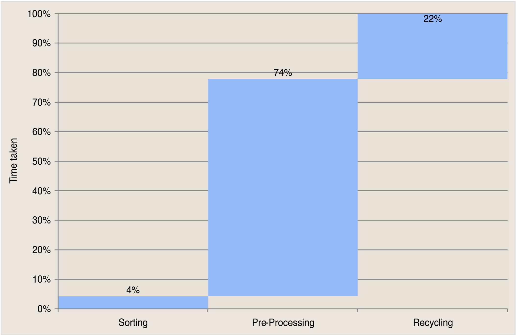
Figure 80: Polyester trial time taken per kg
