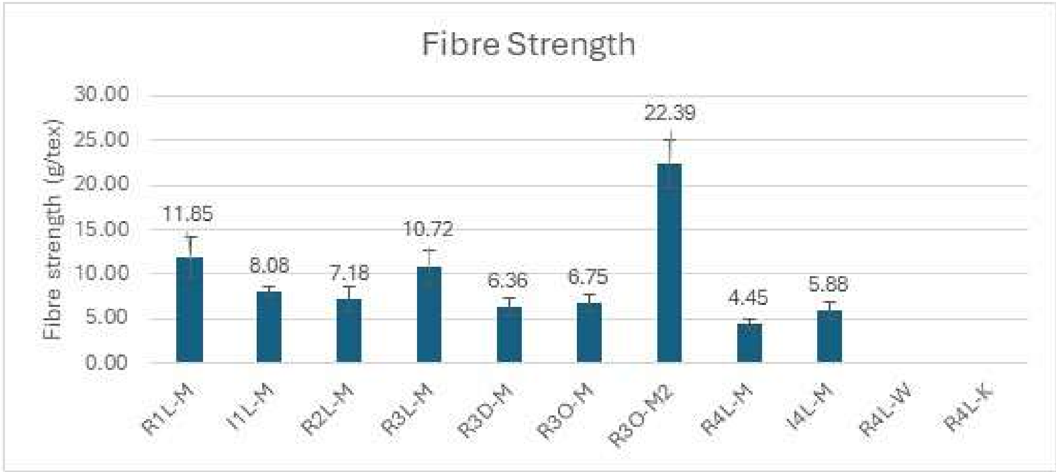
Figure 95: Cotton fibre analysis: Strength
