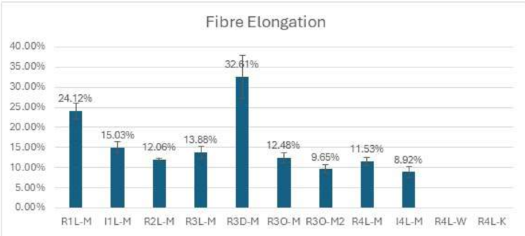
Figure 96: Cotton fibre analysis: Elongation
