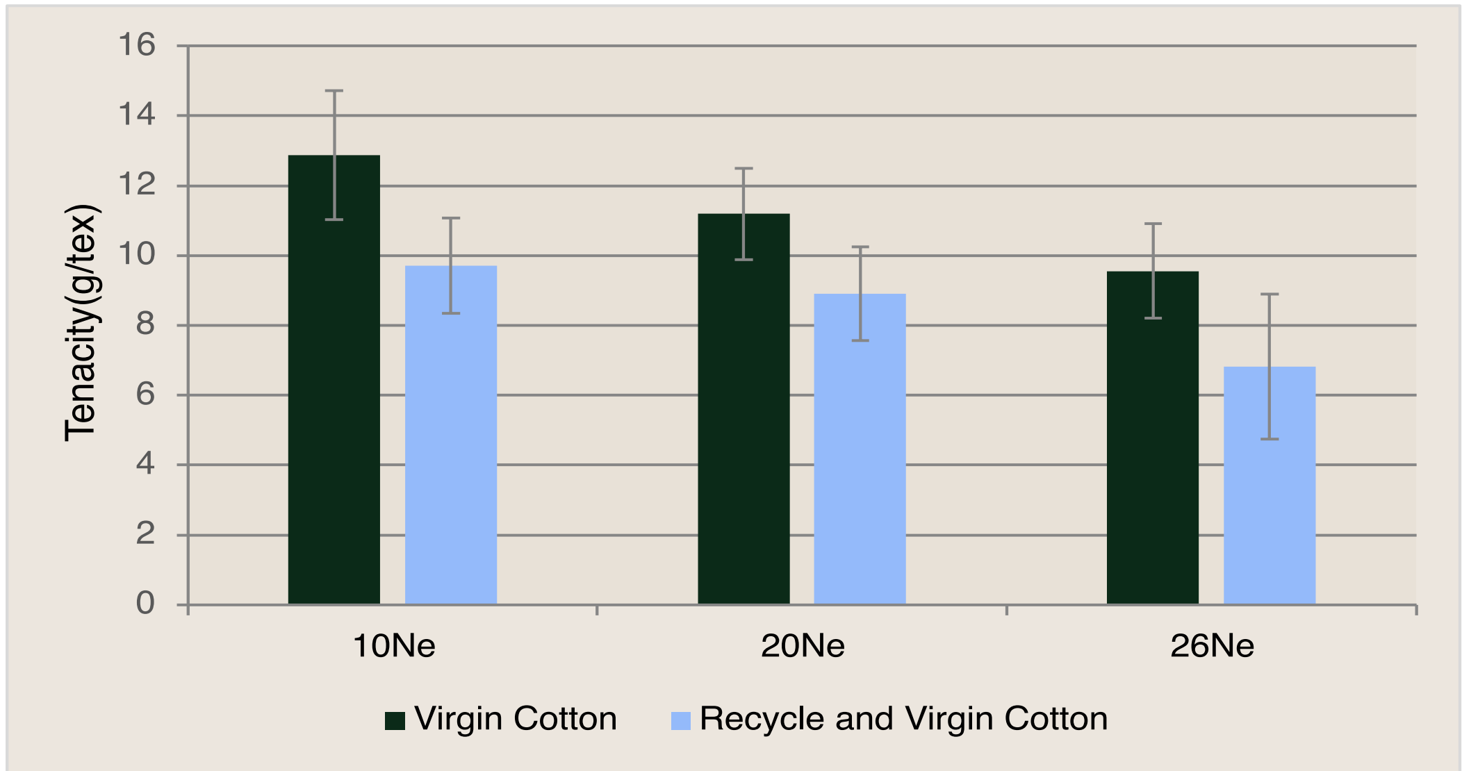
Figure 73: Tensile strength between virgin and recycled blend yarns at 10Ne, 20Ne, and 28Ne
