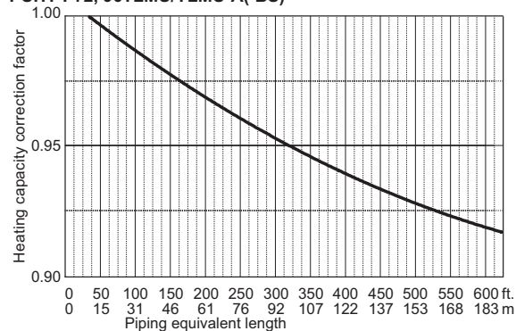
PUHY-P72, 96TLMU/YLMU-A(-BS)
