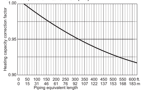
PUHY-P336, 360TSLMU/YSLMU-A(-BS)
