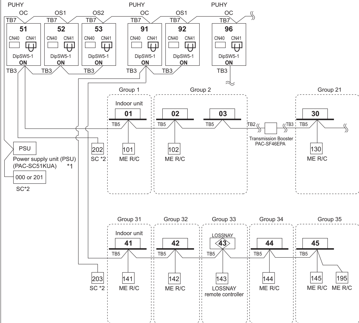
12-4-3-6. ME remote controller, Multi-refrigerant-system, System Controller at TB7 side, LOSSNAY, Booster for long M-NET wiring
