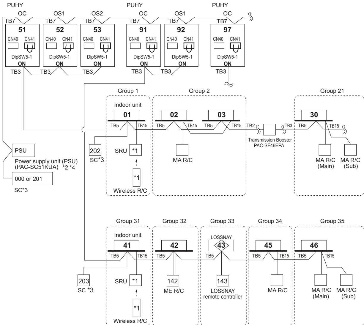
12-4-3-3. MA remote controller, Multi-refrigerant-system, System Controller at TB7/TB3 side, Booster for long M-NET wiring
