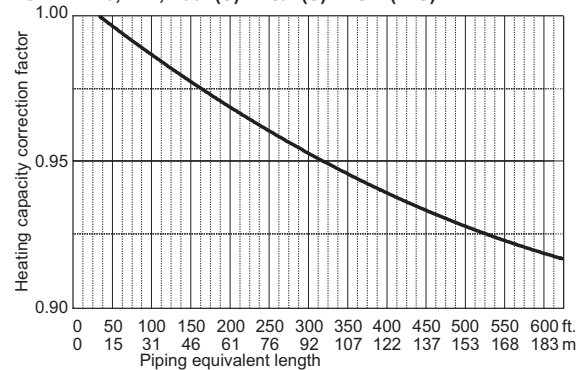
PUHY-P120, 144, 168T(S)LMU/Y(S)LMU-A(-BS)
