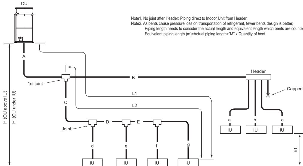
Fig. 13-2-1A Piping scheme
