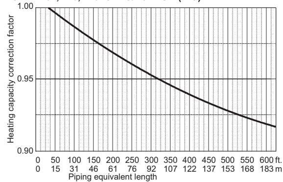
PUHY-P192, 216, 240TSLMU/YSLMU-A(-BS)
