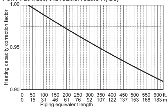
PUHY-P264, 288, 312TSLMU/YSLMU-A(-BS)
