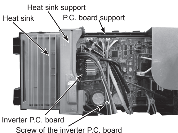
Photo 6-2 (NAXSKH15/18)
