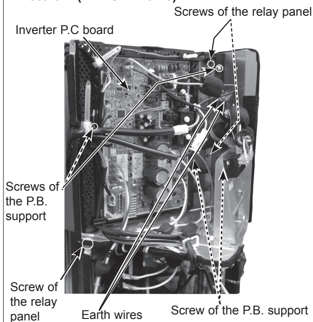
Photo 6-2 (NAXSKH15/18)
