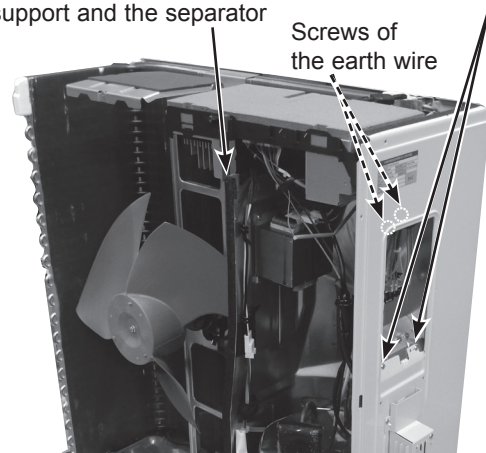
Photo 6-1 (NAXSKH09/12)
