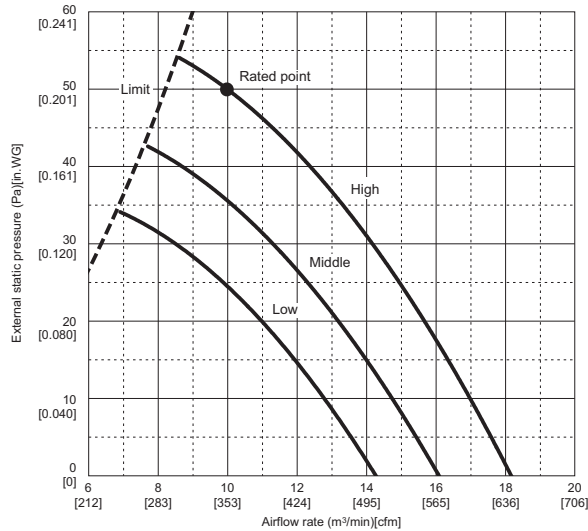
TPEADA0091AA70A (External static pressure 50Pa) 208-230V 60Hz
