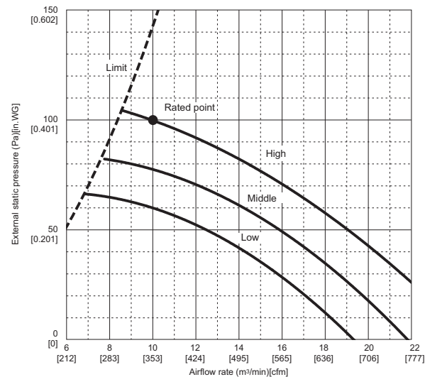
TPEADA0091AA70A (External static pressure 100Pa) 208-230V 60Hz
