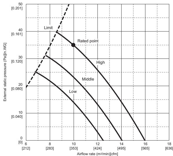
TPEADA0091AA70A (External static pressure 35Pa) 208-230V 60Hz
