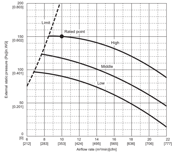
TPEADA0091AA70A (External static pressure 150Pa) 208-230V 60Hz
