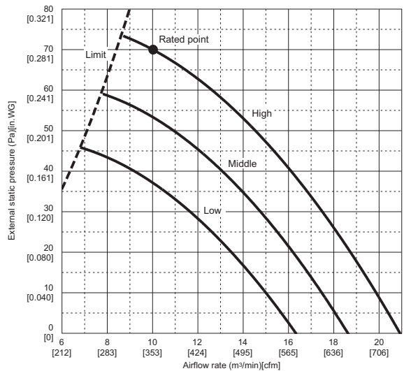
TPEADA0091AA70A (External static pressure 70Pa) 208-230V 60Hz
