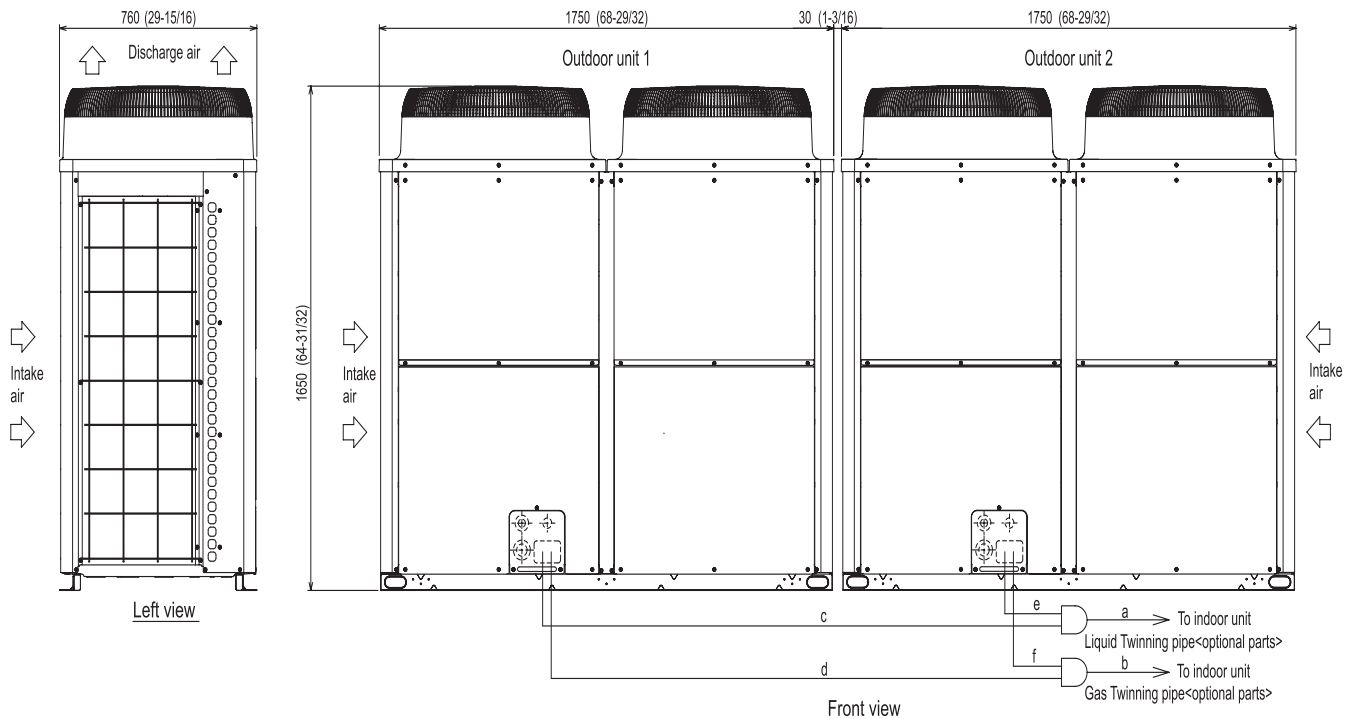
Twinning pipe connection size
