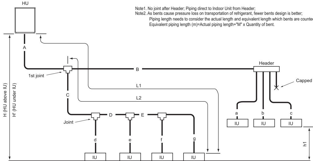
Fig. 12-2-1A Piping scheme
