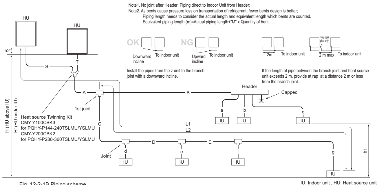
Fig. 12-2-1B Piping scheme
