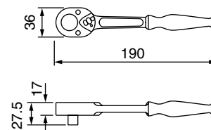
[Fig. 3-2] Ratchet handle/9.5mm (3/8")
