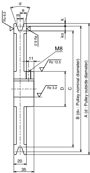
Shape of the pulley (unit:mm)
