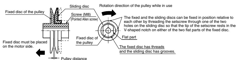
(Figure 1) Variable-width pulley
