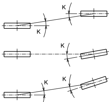
(Figure 1) Pulley's degree of parallelism
