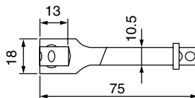
[Fig. 3-1] Extension bar
