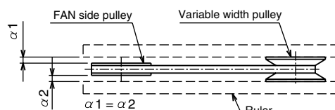
(Figure 2) Adjusting the horizontal alignment of the variable-width pulley
