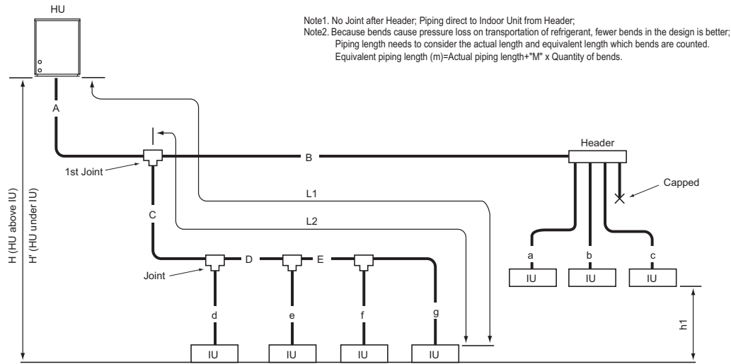
Fig. 3-2-1A Piping scheme
