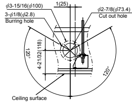
Detail drawing of fresh air intake
