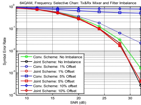
Figure 7. Scenario 1, 64-QAM: Tx & Rx Mixer and Filter Imbalance
