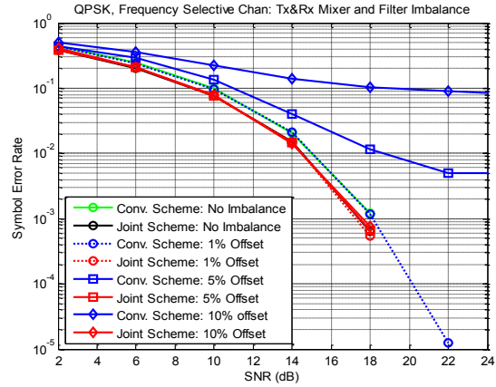
Figure 6. Scenario 1, QPSK: Tx & Rx Mixer and Filter Imbalance
