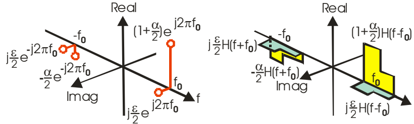
Figure 2. New spectral terms introduced due to imbalance in I-Q mixing
