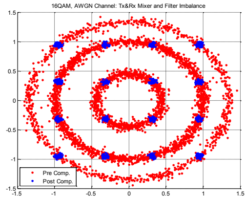
Figure 5. Mixer and Filter Imbalance output at Tx & Rx – 16QAM
