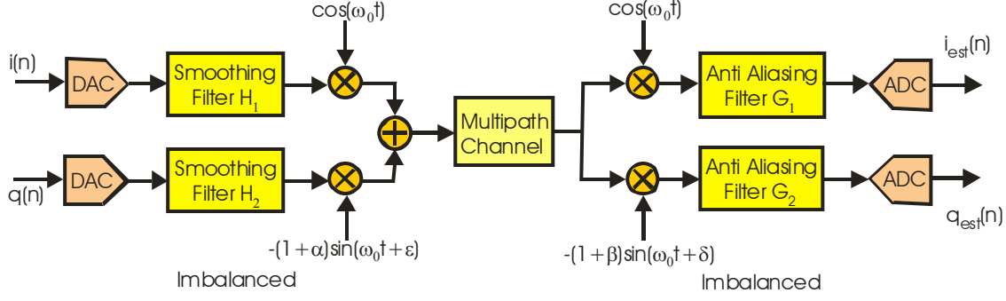
Figure 1. Imbalanced I-Q mixing and filter at Transmitter and Receiver
