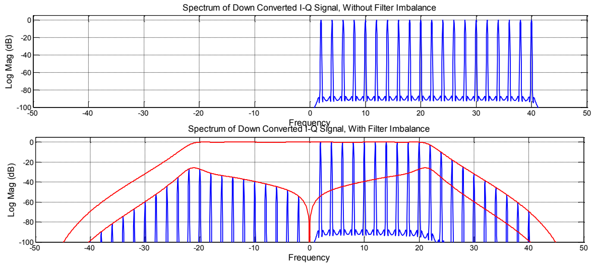
Figure 3. New spectral terms introduced due to imbalance in I-Q Filters
