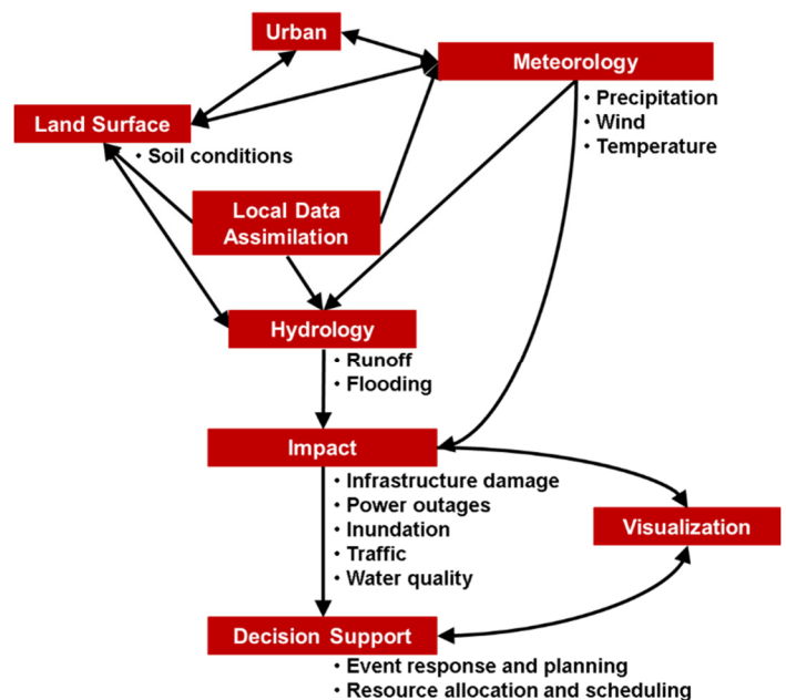
Figure 2 Data flow for coupled models to enable predictions of weather-driven impacts.
