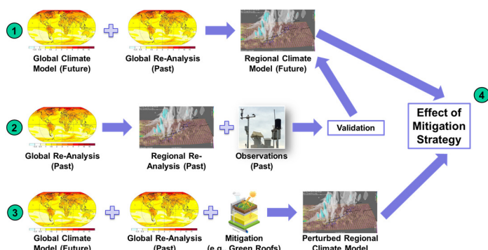
Figure 5 Data flow and processes to apply the PGW method to estimate future climate states
