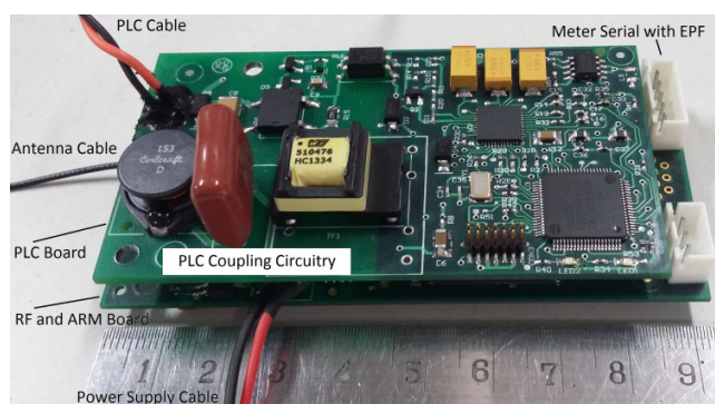
Figure 4. Board stack.
