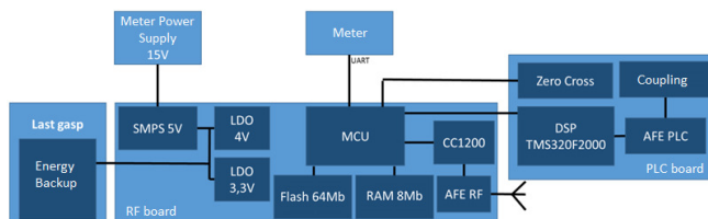
Figure 2 - Diagram of the communication module blocks.
