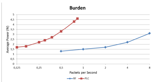
Figure 5. Average burden for RF and PLC.
