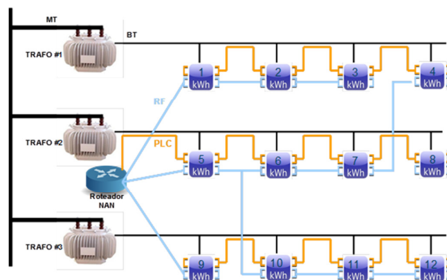
Figure 1. PLC crossing transformers through RF bridges.
