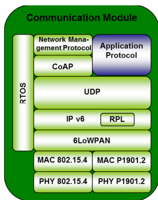
Figure 3. Protocol stack.
