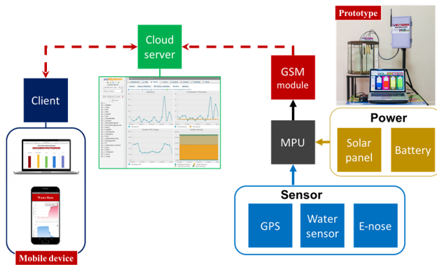
Figure 2. Block diagram of IoT indirect BOD monitoring system based on E-nose technology
