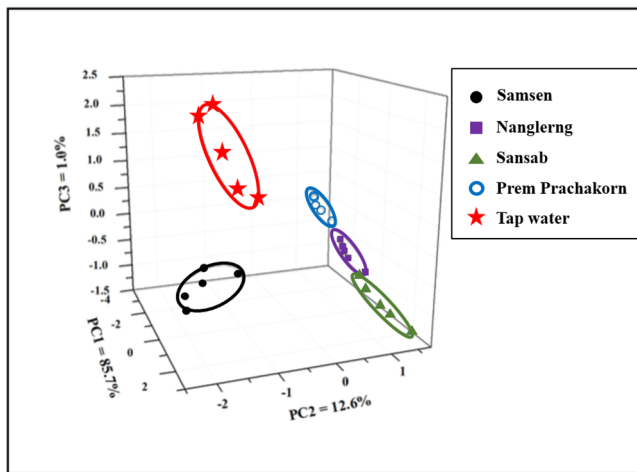
Figure 3. 3D PCA result of water sample from four different source compare with tap water.
