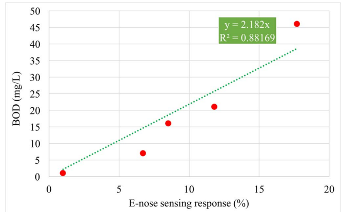
Figure 4. Correlation plot between BOD value and electronic nose sensing response
