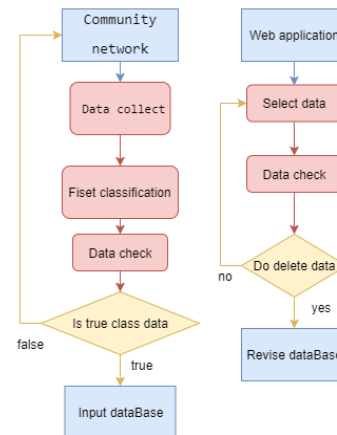
Figure 4: System flowchart
