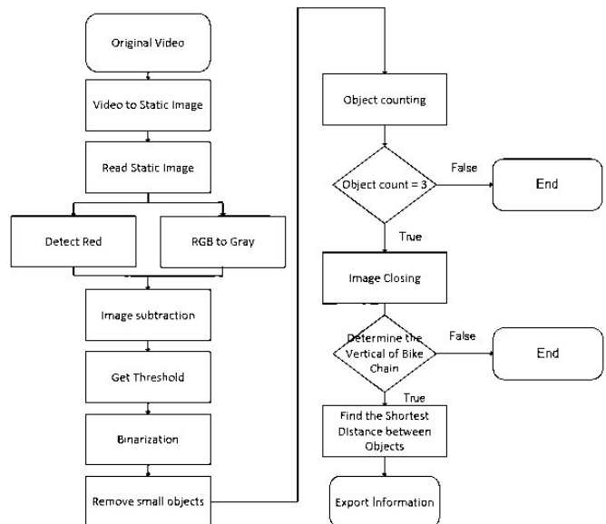
Fig. 2. The identification algorithm of bicycle objects.
