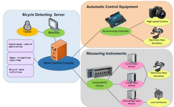
Fig. 1. System structure diagram
