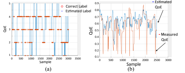
Fig. 2 An example of estimation results of (a) HMM and (b) RNN with LSTM. In case of HMM, concordance rate is 0.497 and correlation coefficient is 0.371. In case of RNN, concordance rate is 0.3 and correlation coefficient is 0.196.
