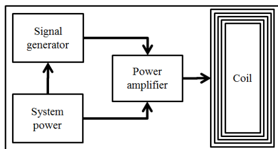
Fig.1 Block diagram of the ELF-EMF system
