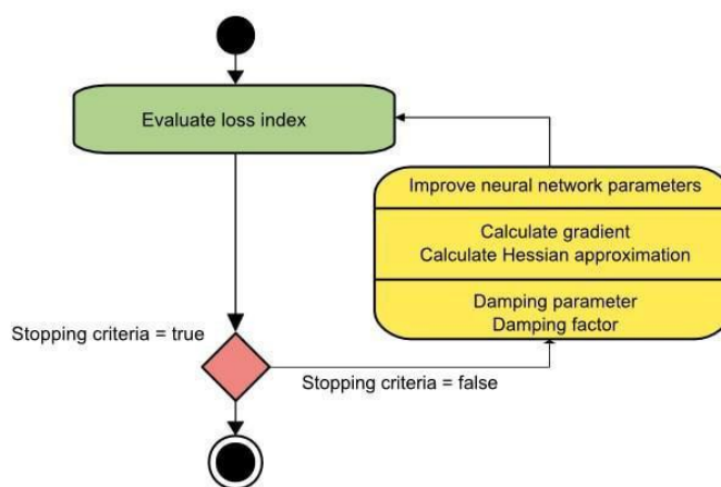
Fig 1: Working of the Levenberg-Marquardt algorithm
