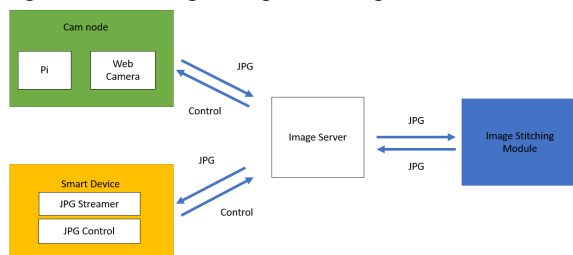
Figure 1: System Architecture
