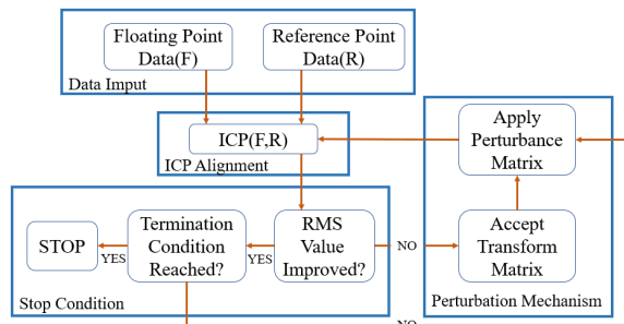
Fig 2: Flowchart of Improved Alignment (IA) Algorithm
