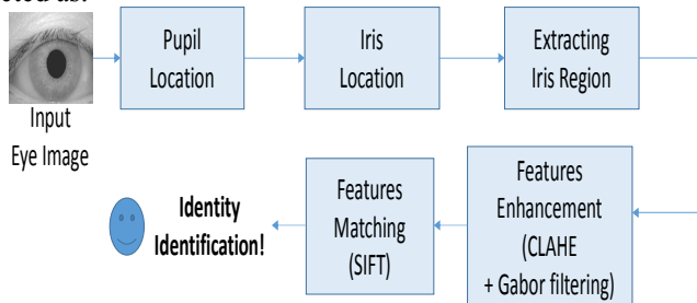
Fig. 1 The proposed processing flow for iris-based identity identification
