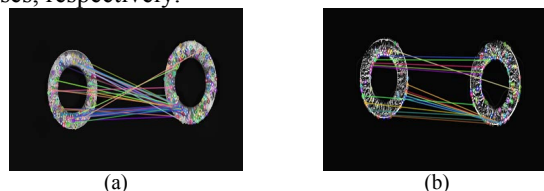
Fig. 6 Features matching results by (a) CLAHE and (b) CLAHE +Gabor filtering processes
