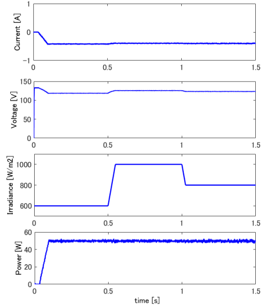
Fig. 4 Current, voltage responses, and output power of the PV with varying irradiance
