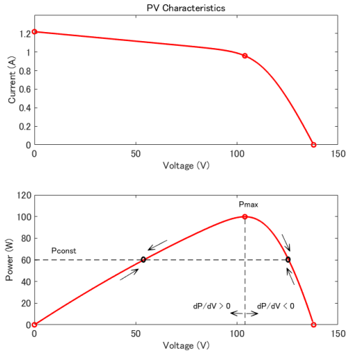
Fig. 3. Voltage-current and voltage-power characteristics of PV
