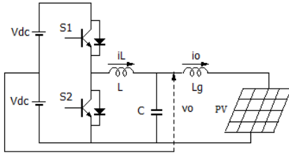
Fig. 2. PV connected inverter circuit.
