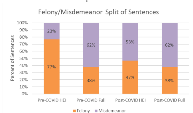
Fig. 3. Felony/Misdemeanor Split of Sentences. Felony charges dominated HEI usage pre-COVID.
