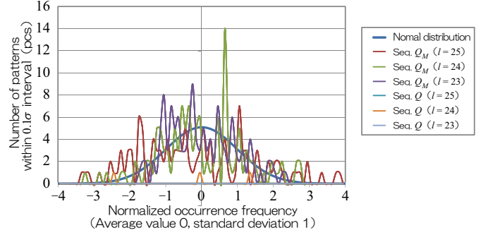
Fig. 1. Distribution of sequence bit patterns.
