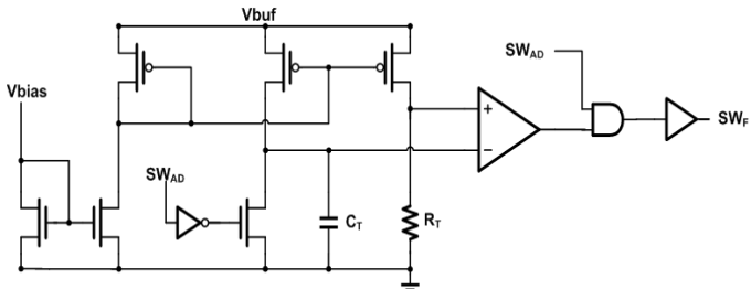
Fig. 5 Schematic of the precision timer control of the flip switch.
