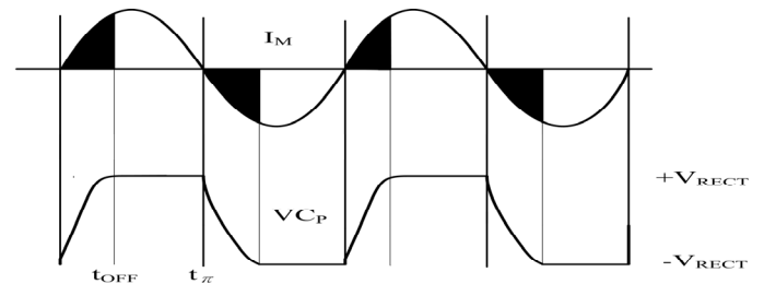
Fig. 2 Simulated of the voltage and current waveforms for a full-bridge rectifier connected to a piezoelectric energy harvester.
