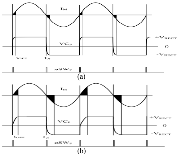
Fig. 6 Simulated voltage and current waveforms: (a) Parallel-SSHI rectifier and (b) Switch-Only rectifier connected to a piezoelectric energy harvester.
