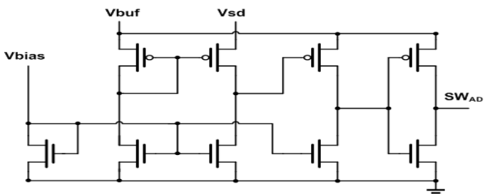
Fig. 4 Schematic of the common-gate comparator.
