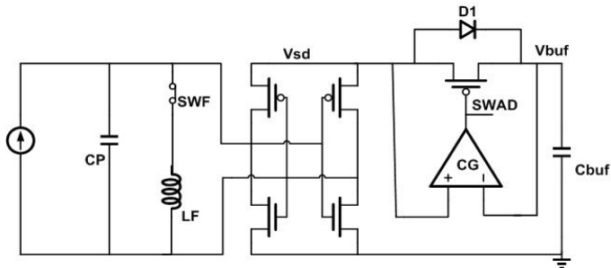
Fig. 3. Schematic of the Parallel-SSHI interface together with the active rectifier.
