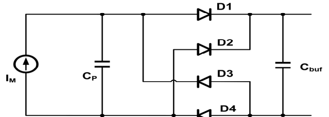
Fig. 1 Schematic of the Full-Bridge Rectifier circuit.
