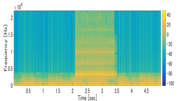
Fig 2. Spectrogram of unknown data (wind noise + horn)
