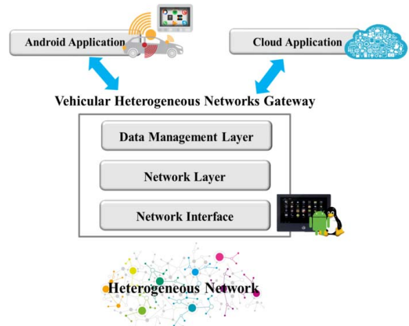
Fig. 1. The proposed IVI platform (vehicular heterogeneous networks gateway) for managing heterogeneous networks information exchange.
