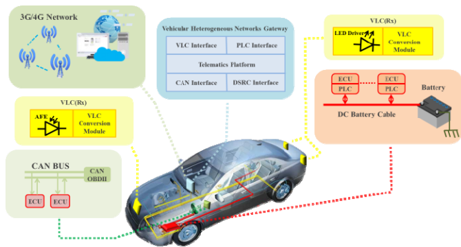
Fig. 2. System architecture of the proposed IVI platform for integrating heterogeneous networks interconnection.
