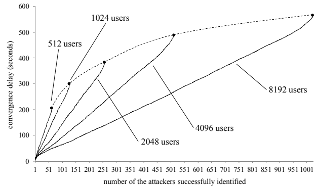
Figure 5 - convergence delay for different number of users
