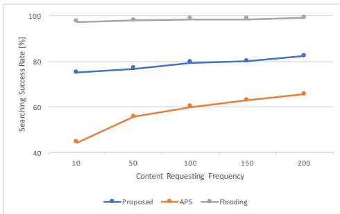
Fig. 1. Relationship between Content Request Frequency and Searching Success Rate.
