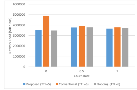
Fig. 2. Relationship between Churn Rate and Total Network Load.
